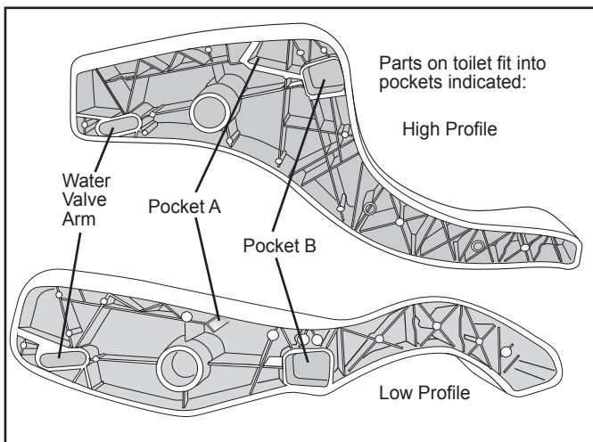
FIGURE 2 - PEDAL REATTACHMENT
